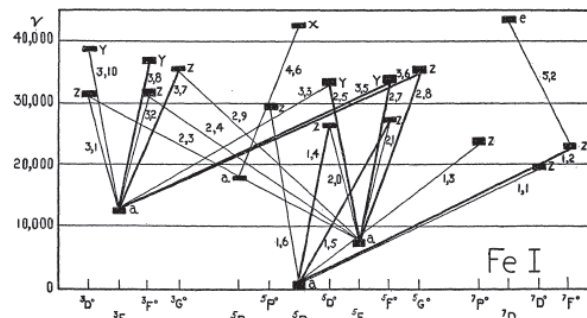
Figure 9: Grotian diagram showing the energy levels of iron that give rise to multiplets identified in meteor spectra (after Millman, 1932: 137).
