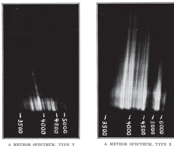
Figure 11: Millman's classification of meteor spectra. On the left is Type Y, with strong calcium H and K lines, and on the right Type Z, which is dominated by iron (after Millman, 1936b: 385).
